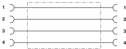
Contact assignment of the M12 sockets
